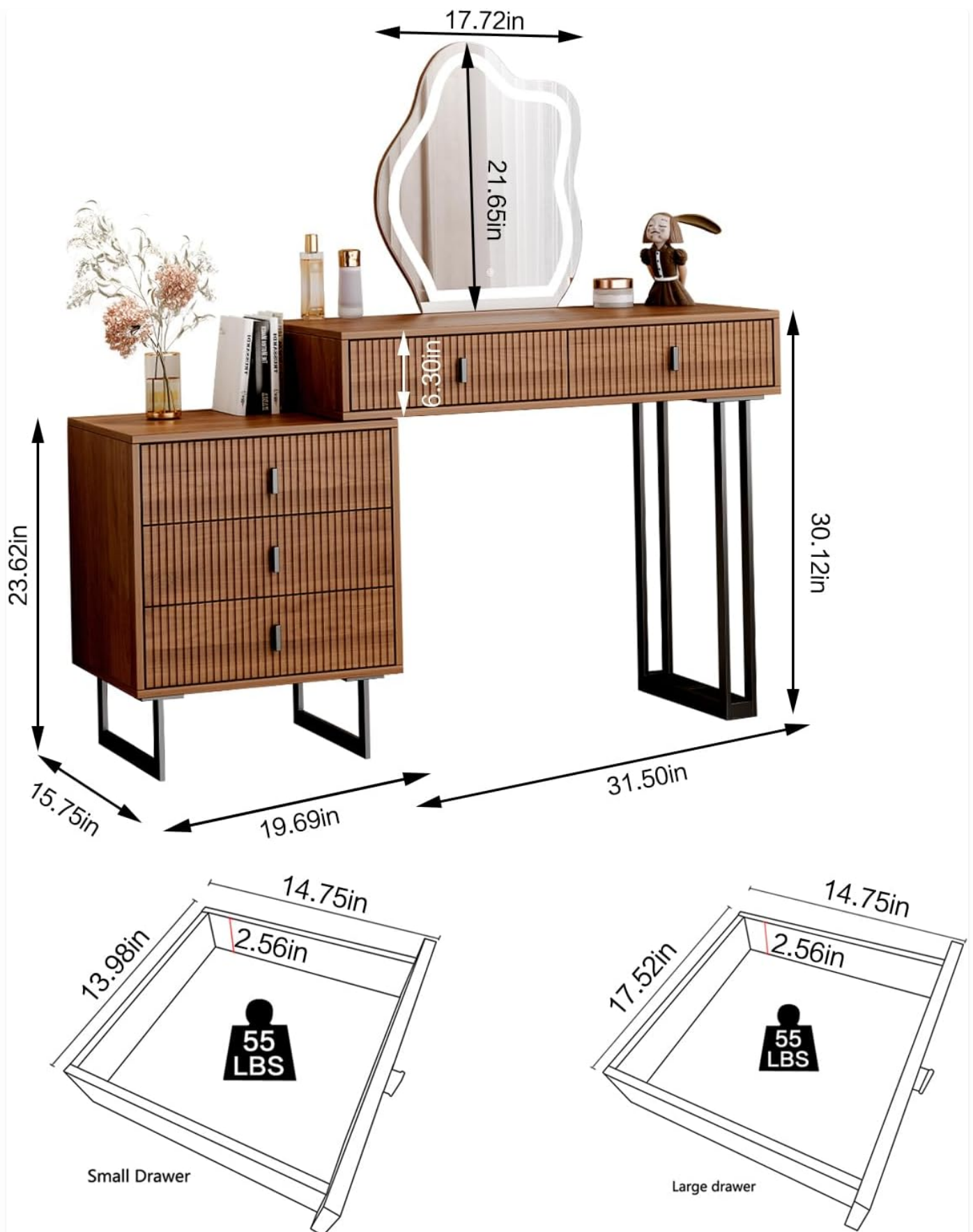
Detailed dimensions of the Ieejdn Brown Vanity Desk, including drawer capacities.
