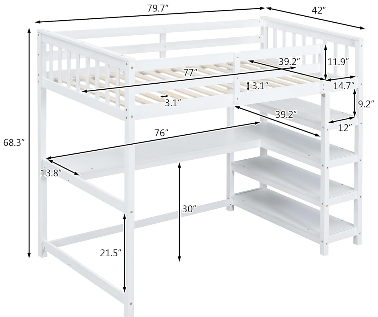
Image: Detailed dimensions of the loft bed, desk, and shelves.
