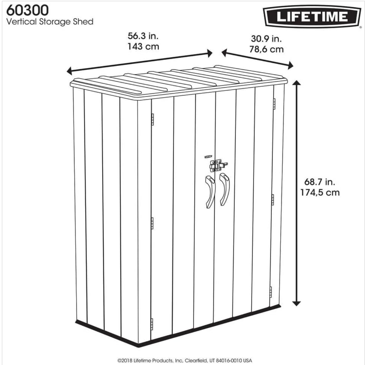
Image: Technical drawing showing the dimensions of the Lifetime Vertical Storage Shed: 56.3 inches (143 cm) width, 30.9 inches (78.6 cm) depth, and 68.7 inches (174.5 cm) height.
