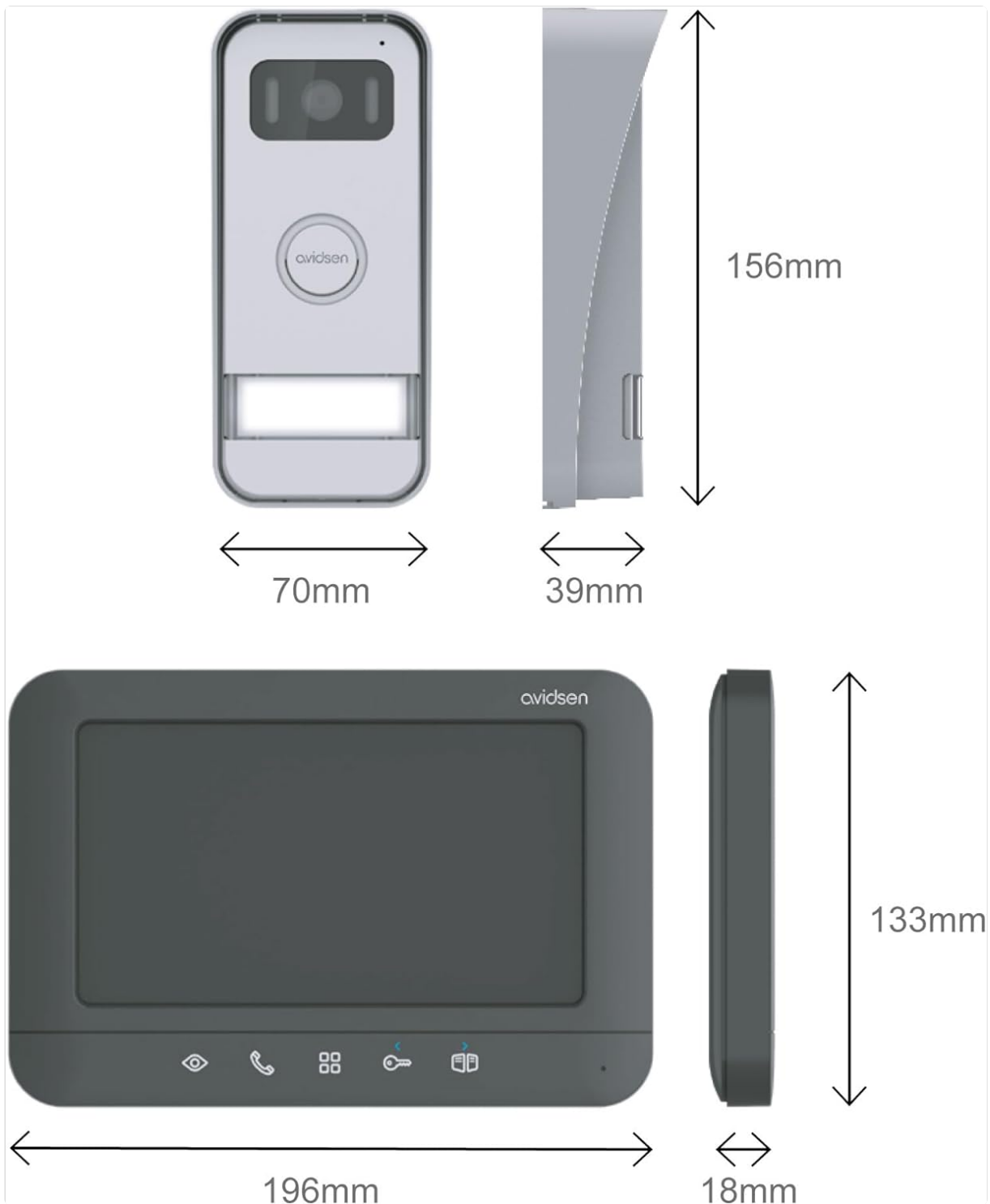
Figure 6.1: Dimensions of the Avidsen PRIMA monitor and outdoor unit.
