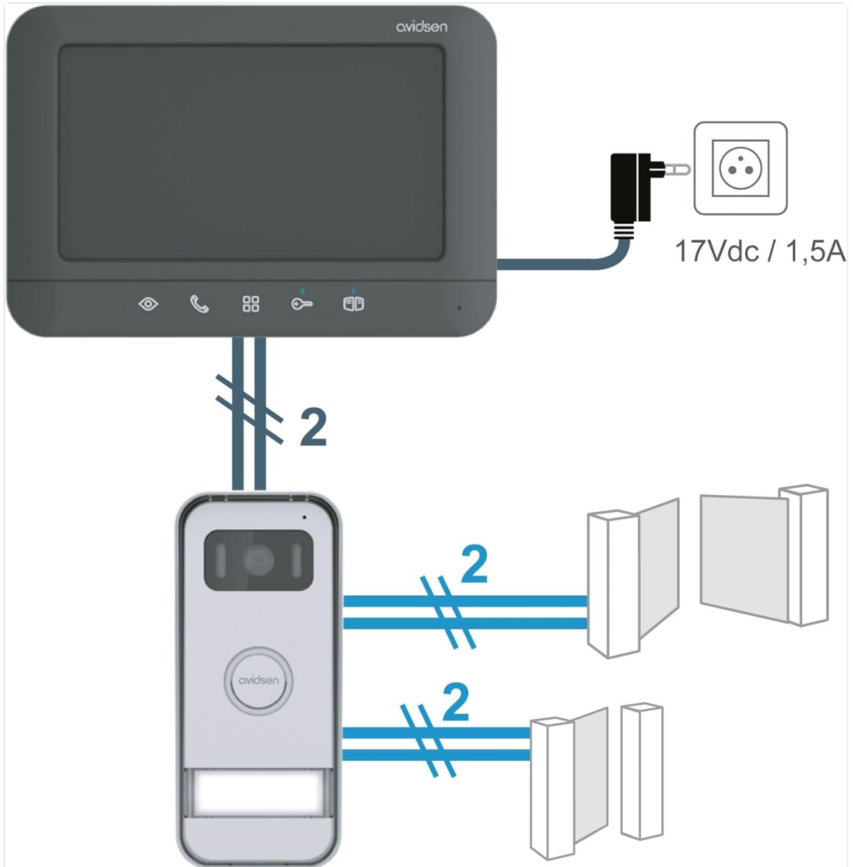
Figure 2.1: Wiring diagram illustrating the 2-wire connection between the monitor and outdoor unit, and the dual control connections for a gate and pedestrian gate.
