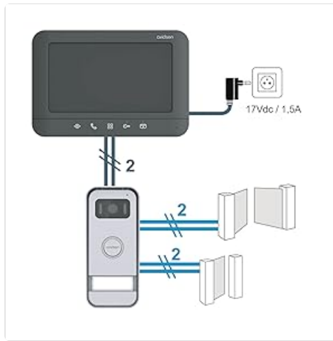
Figure 2.2: Example of outdoor unit installation on a wall.
