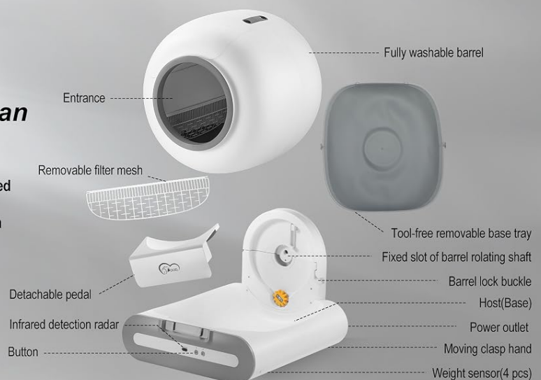
Figure 2: Exploded view of the DOEL Smart Cat Litter Box, highlighting key components such as the washable barrel, removable filter, detachable pedal, and the base unit with sensors.
