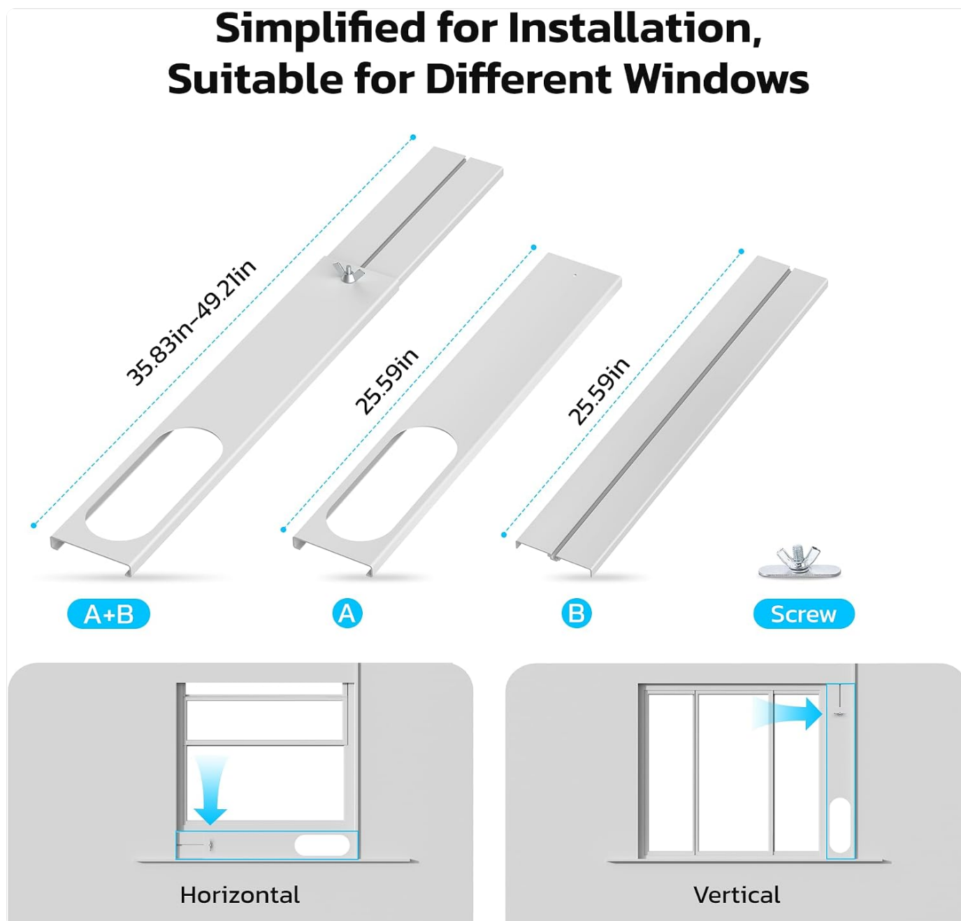
Figure 3: Detailed view of the window kit components and instructions for installing in both horizontal and vertical window types.
