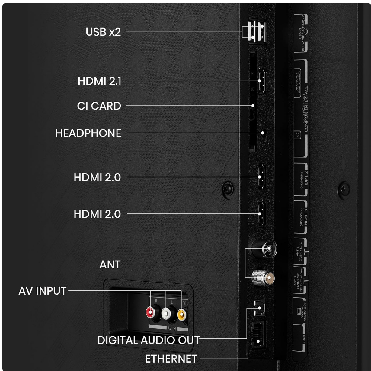
Image: Detailed view of the rear connectivity panel of the Toshiba TV, highlighting ports such as USB x2, HDMI 2.1, CI Card slot, Headphone jack, HDMI 2.0 x2, ANT, AV Input, Digital Audio Out, and Ethernet.
