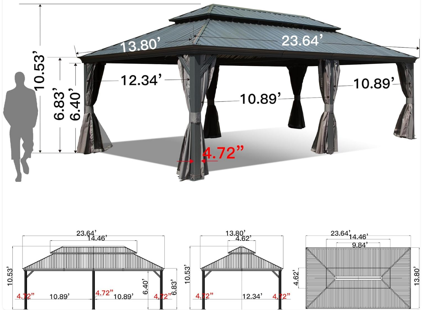
Image 8.1: Dimensional overview of the Domi Gazebo.
