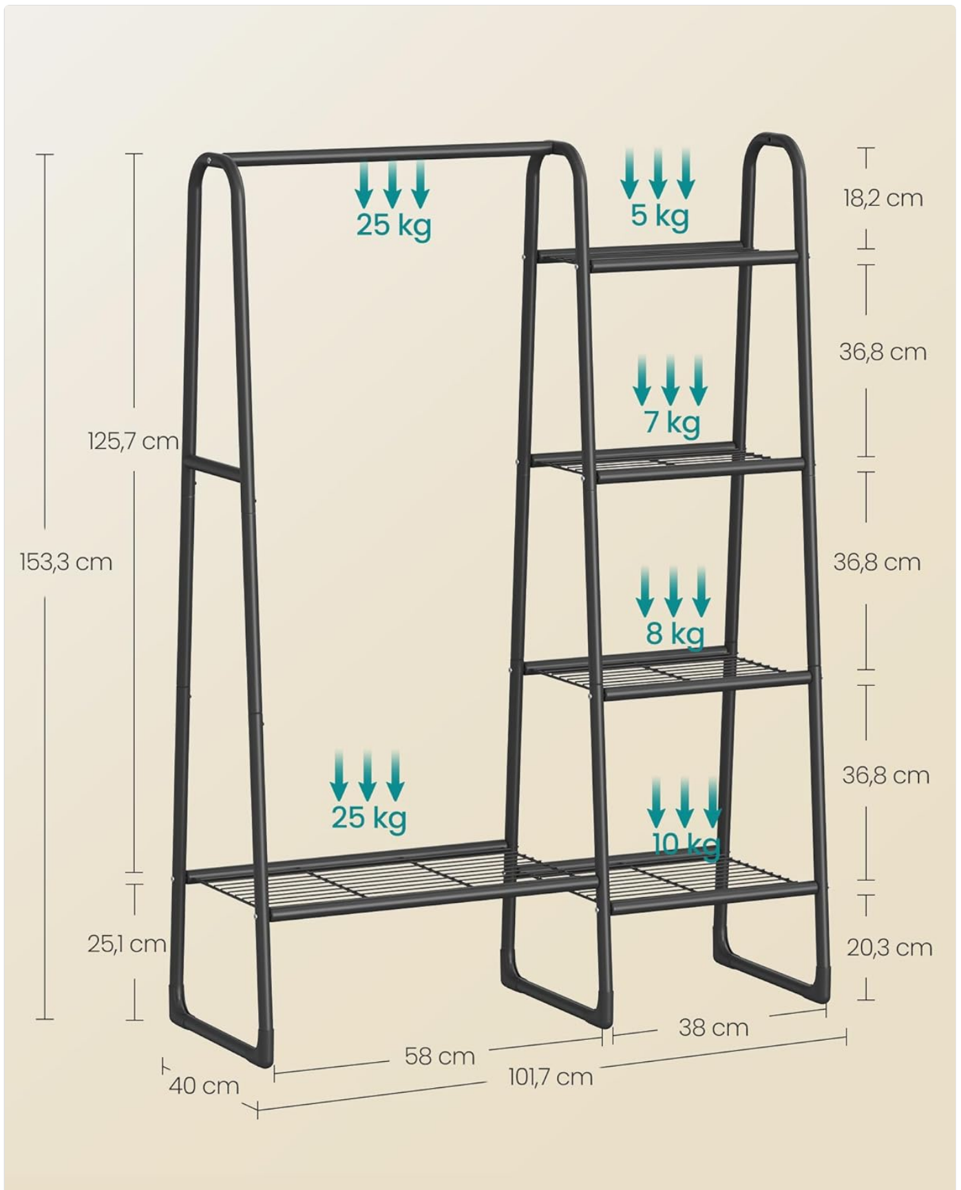
Figure 7: Detailed diagram illustrating the dimensions and individual weight capacities for the hanging bar and each shelf.
