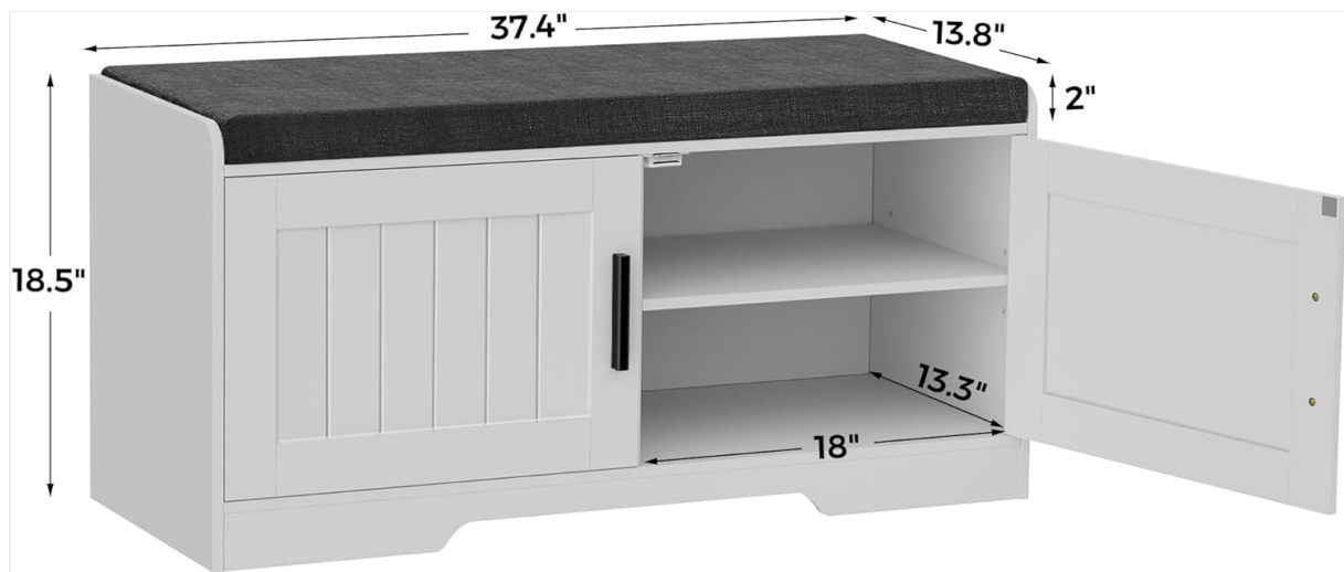
Image 8.1: Detailed product dimensions.
