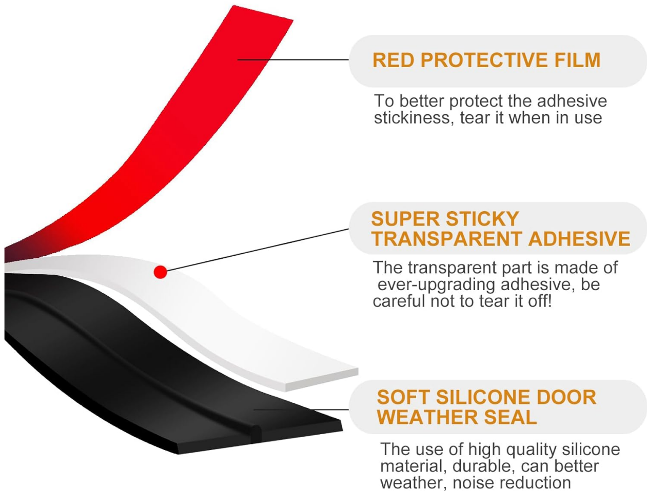
Figure 4.2: Three layers of high-quality material.
