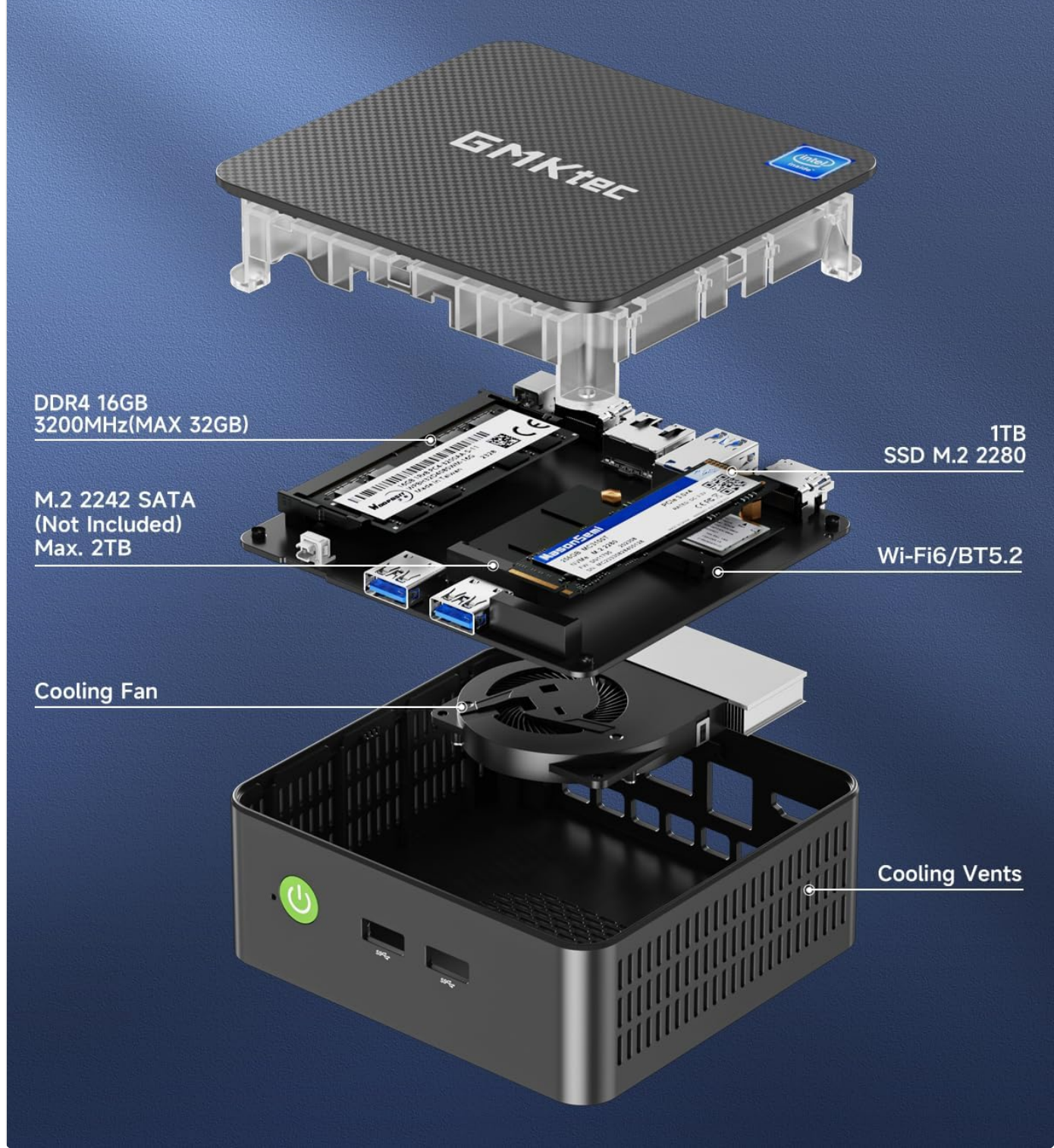
Image: Internal layout and upgrade options for the GMKtec G3 Plus Mini PC.
