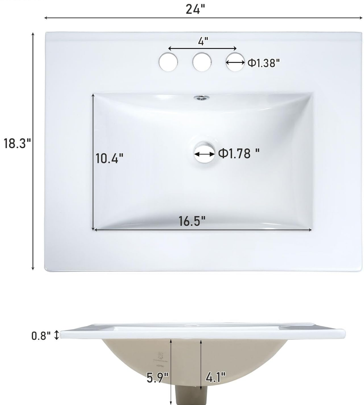
Image 4.2: Ceramic Sink Dimensions.
