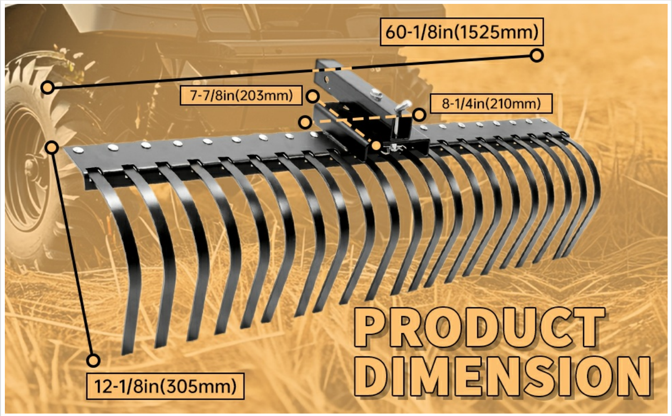
Figure 8.1: Product Dimensions. This image provides a detailed view of the landscape rake's dimensions, including its overall width of 60-1/8 inches (1525mm) and height of 12-1/8 inches (305mm).
