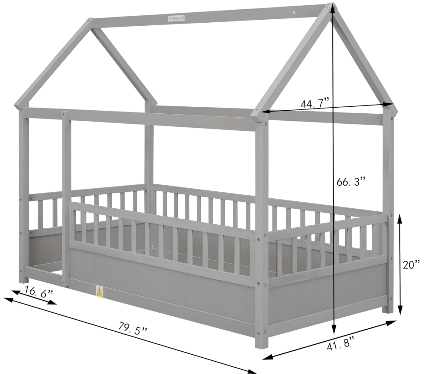
Figure 2.1: Mirightone Twin Size Grey Wooden Floor Bed Dimensions
