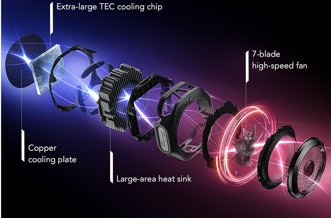
Image: Exploded view showing the copper cooling plate, extra-large TEC cooling chip, large-area heat sink, and 7-blade high-speed fan.
