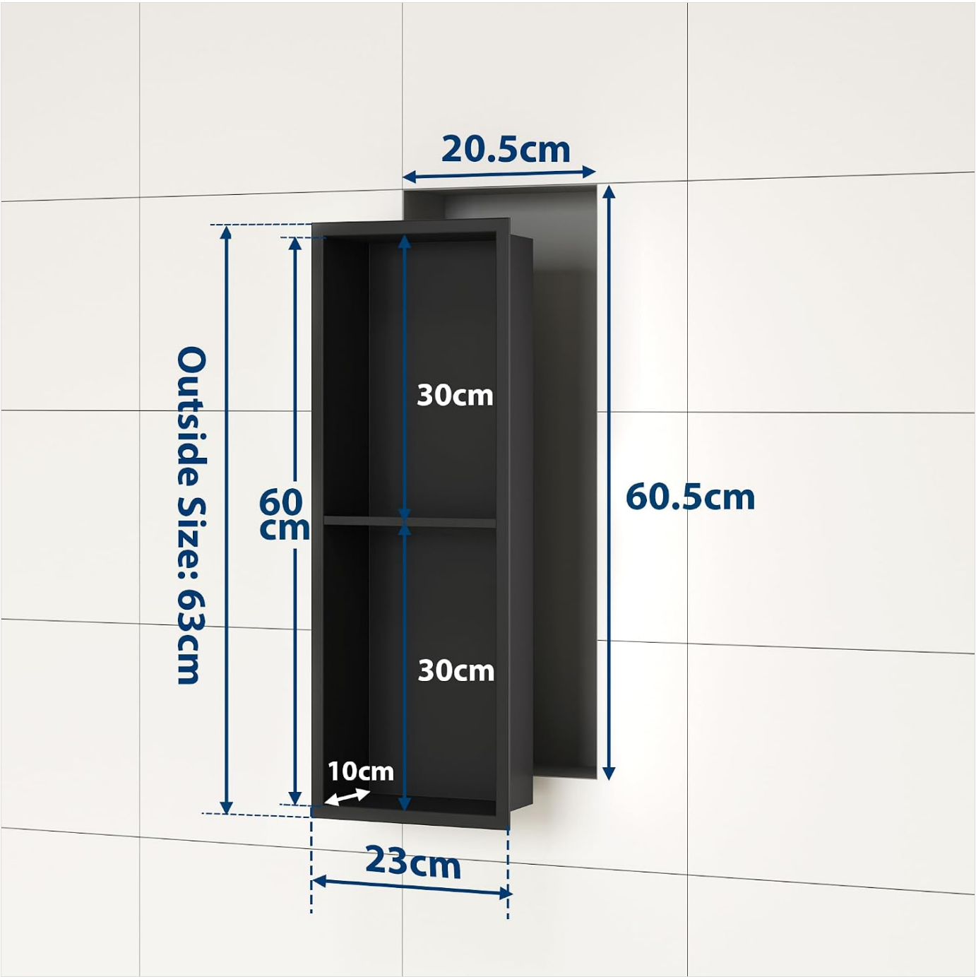
Image 2: Detailed dimensions of the shower niche.
