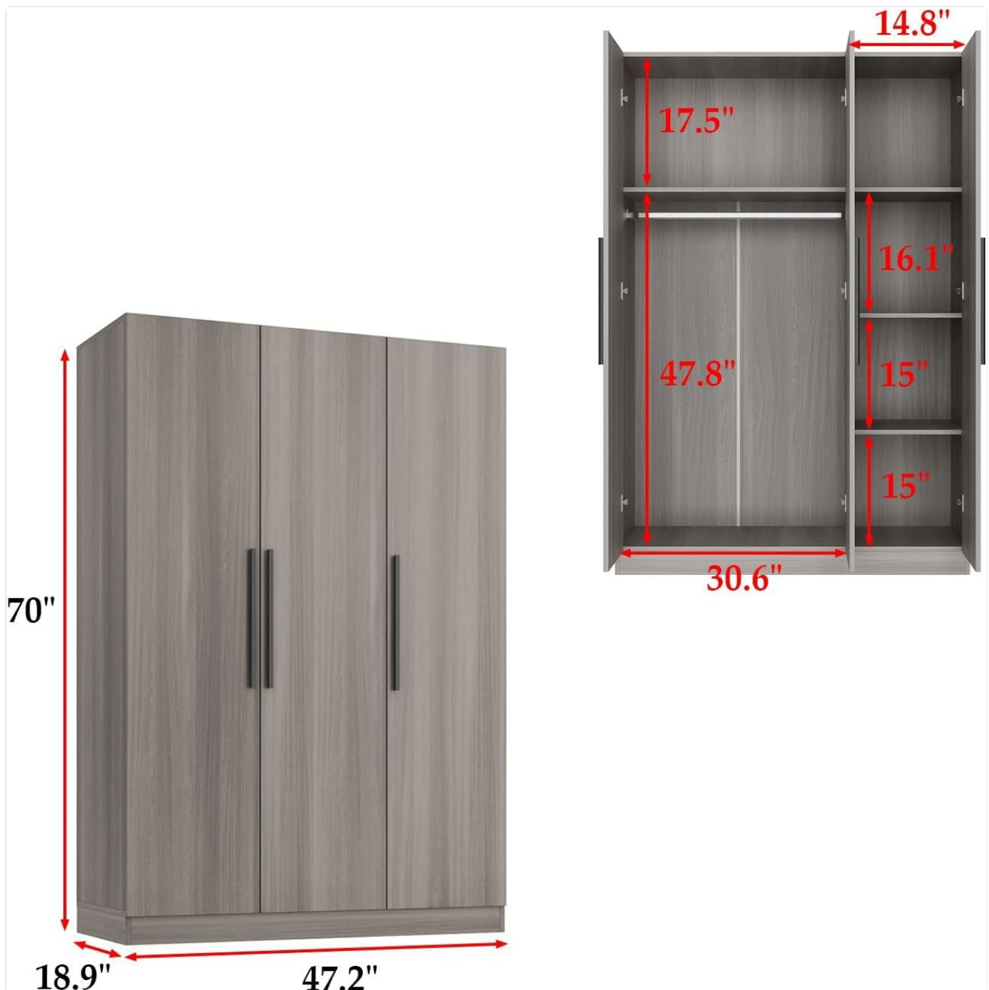
Figure 2: Overall and internal dimensions of the armoire.
