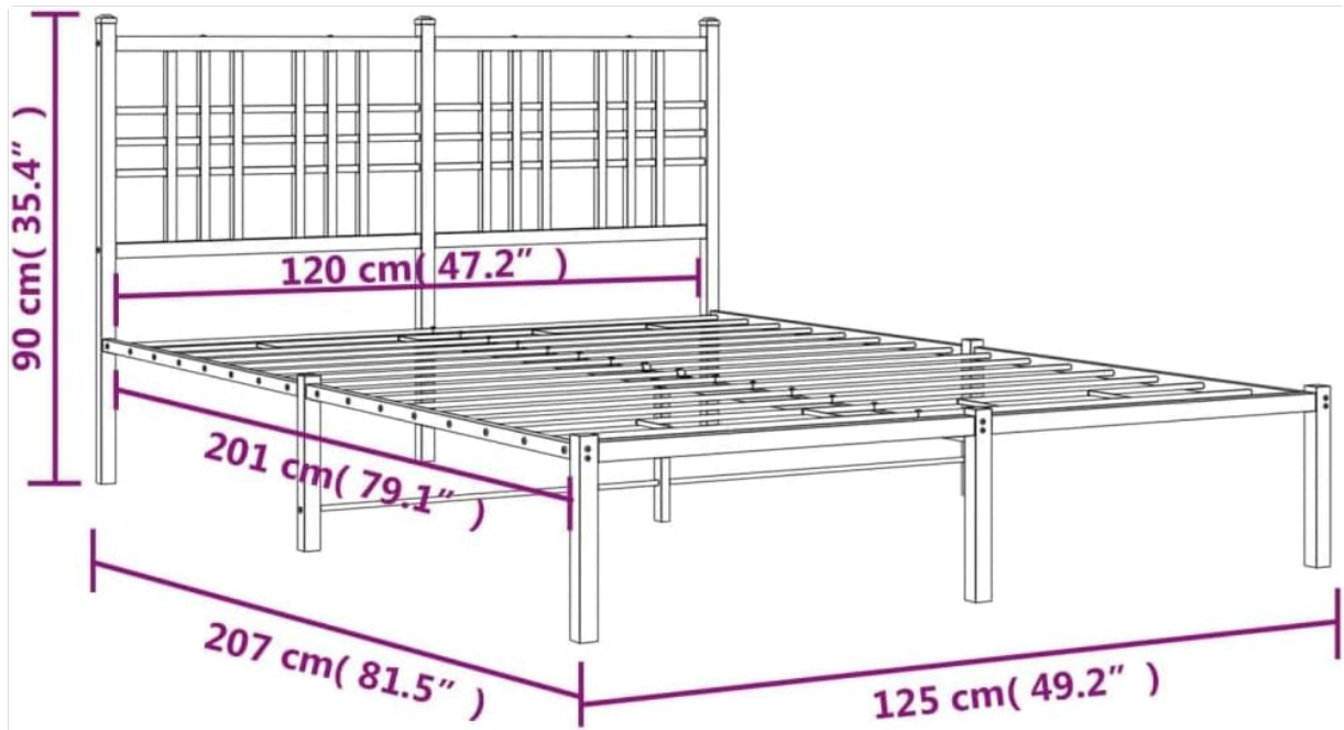
Image 4.1: Dimensional diagram of the vidaXL Full Bed Frame.
