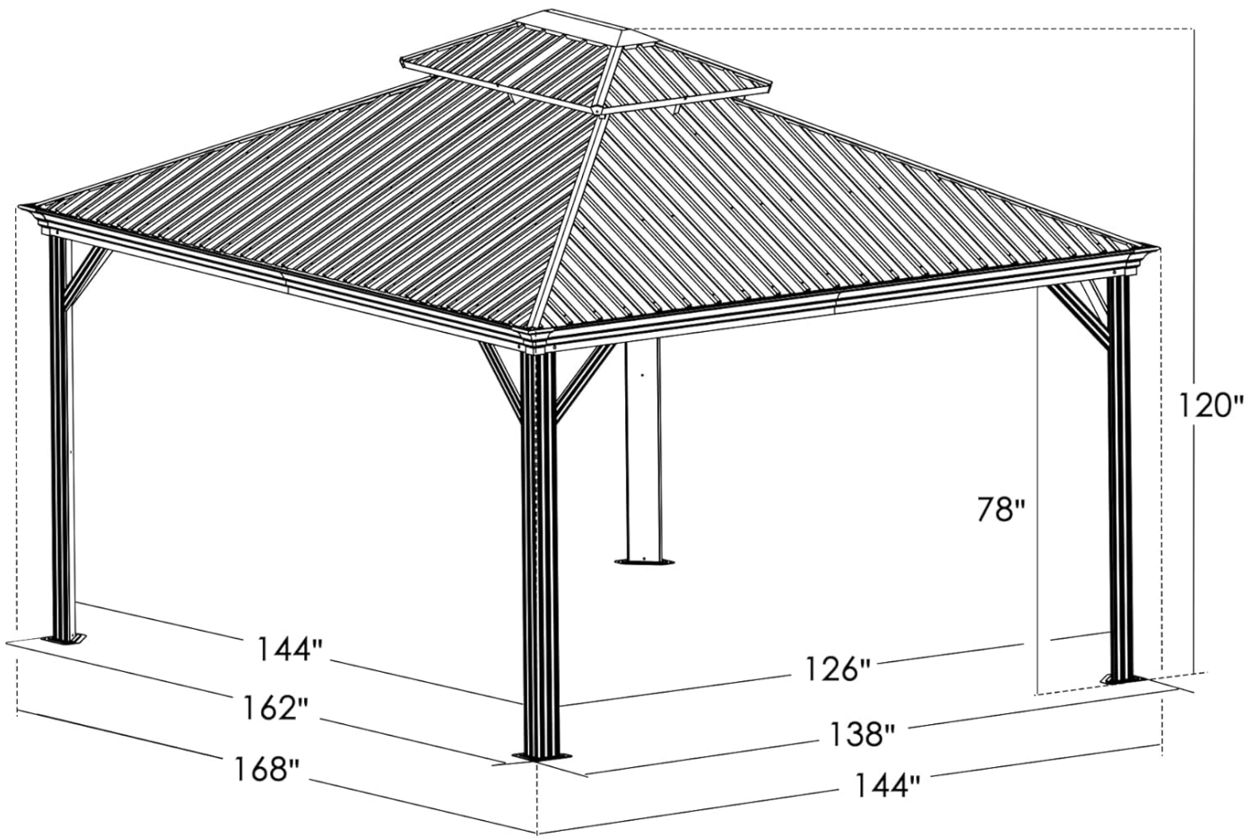
Figure 8.1: Detailed dimensions of the Kozyard Apollo 12'x14' Gazebo.
