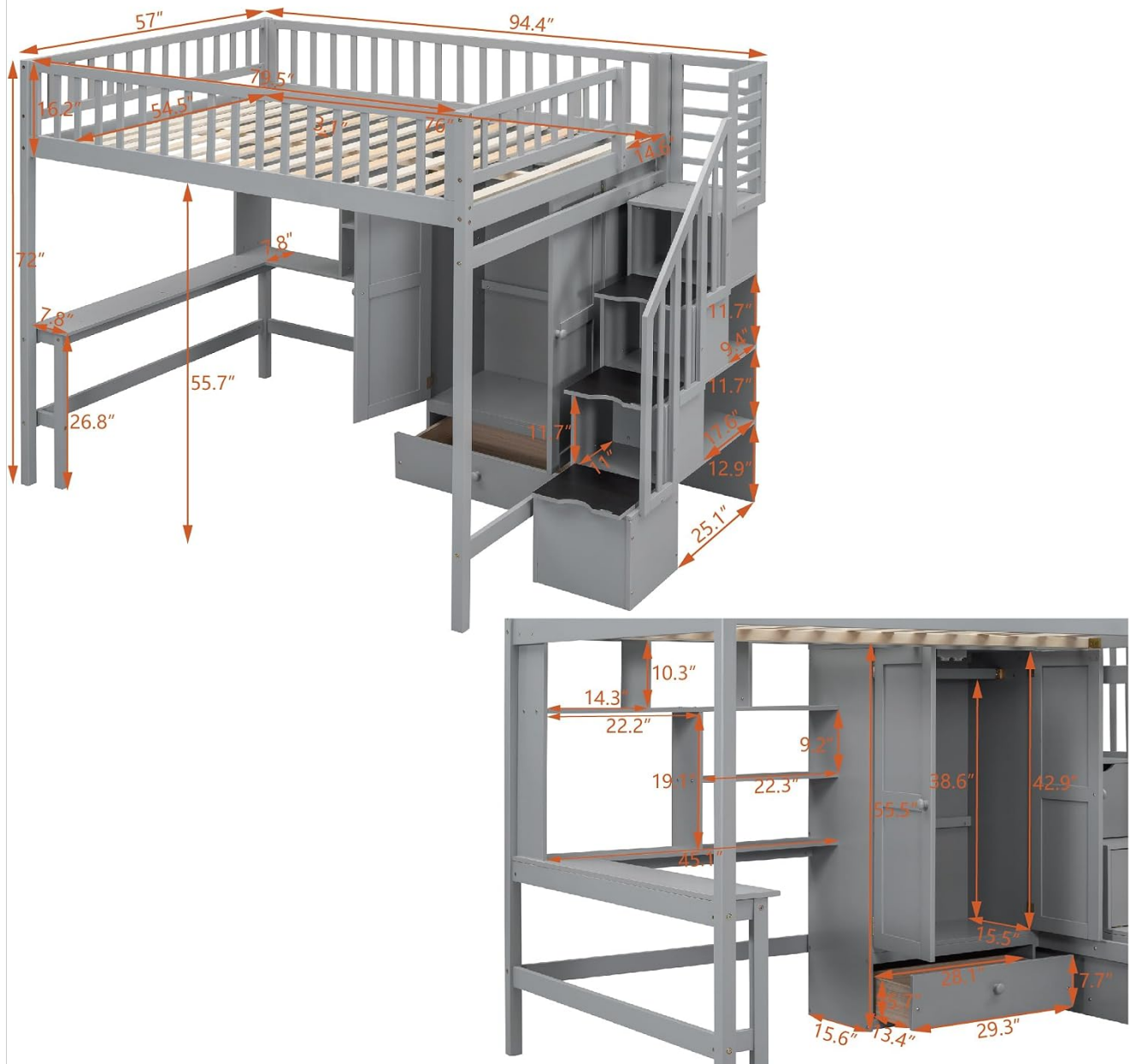
Image 2.1: Dimensional drawing of the BIADNBZ Wooden Full Size Loft Bed. This diagram illustrates the overall length, width, height, and specific measurements of key components like the desk, wardrobe, and staircase storage.
