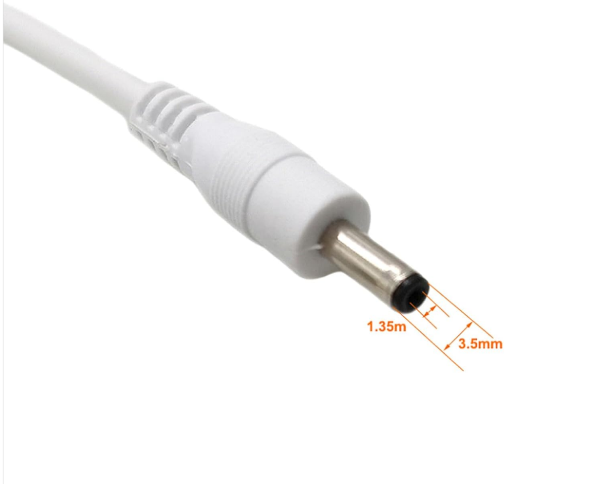
Image: A close-up view of the DC round charging port, indicating its dimensions: 1.35mm inner diameter and 3.5mm outer diameter.
