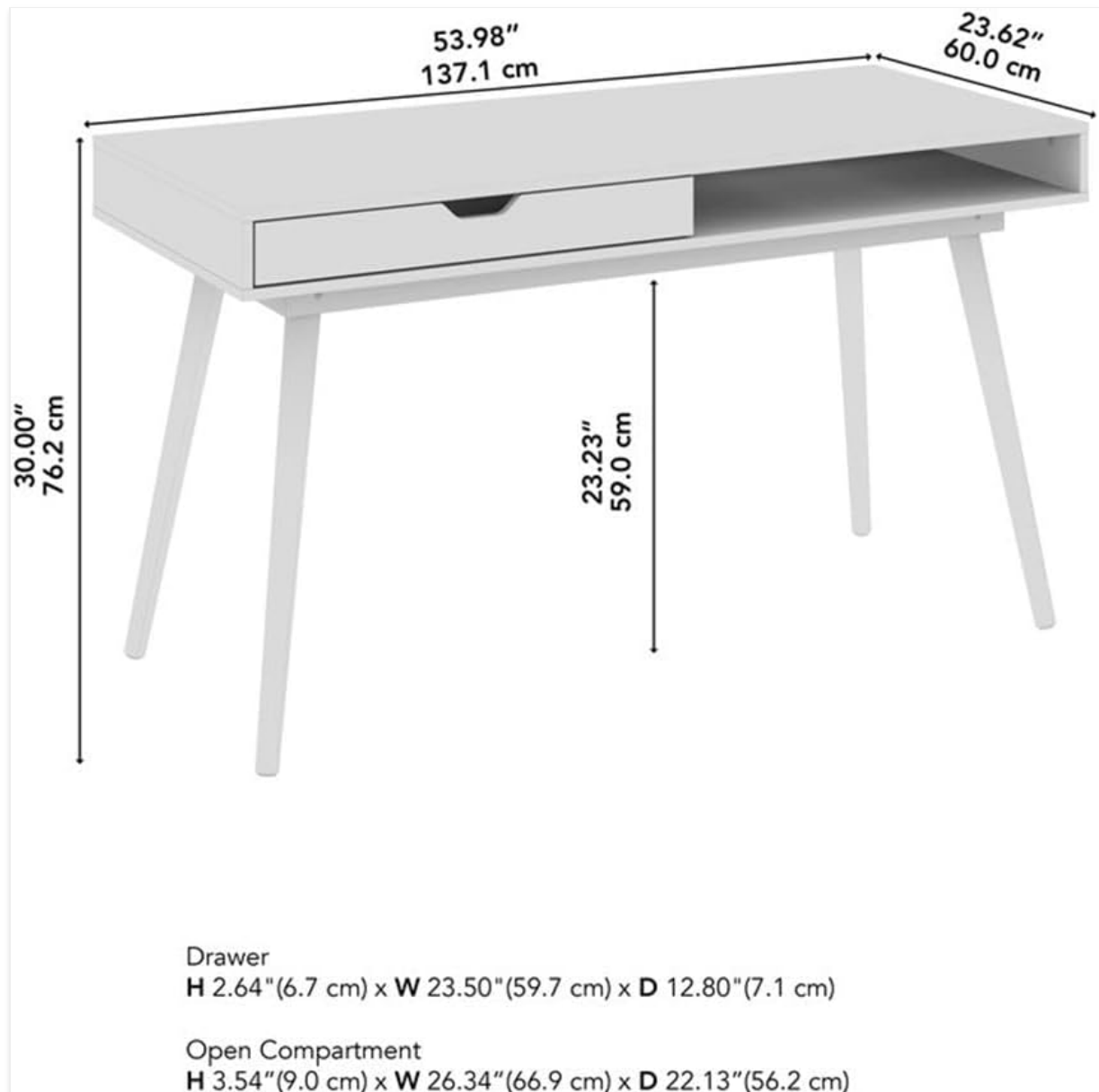
Image 2: Dimensional diagram of the Nora Writing Desk, illustrating overall measurements and internal storage dimensions for the drawer and open compartment.
