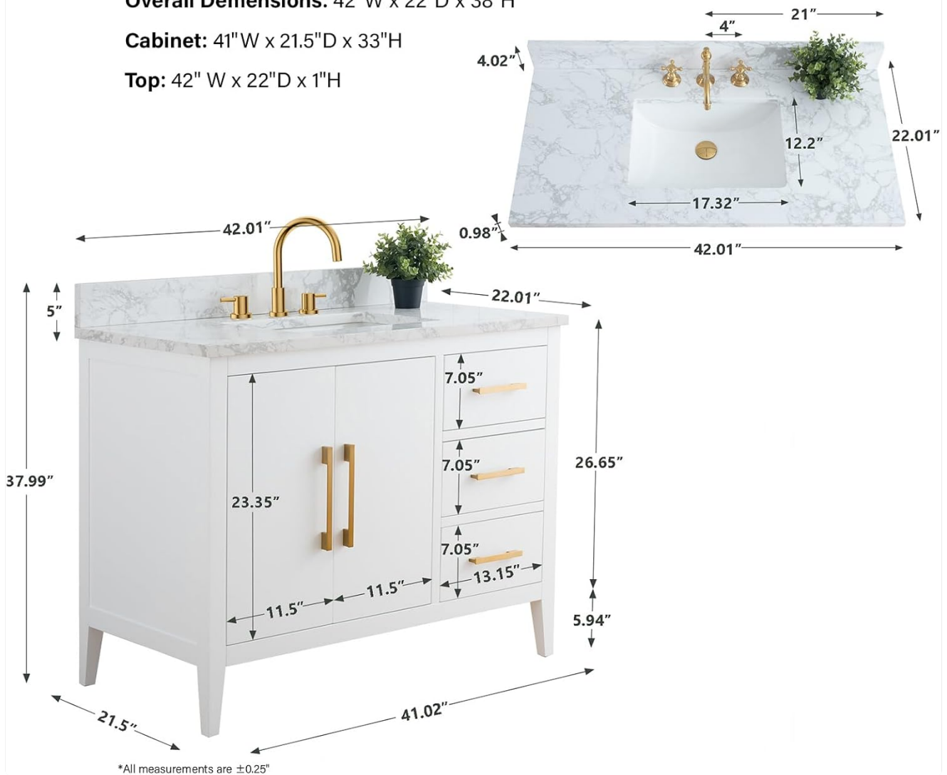
Image 5: Dimensional drawing of the vanity.
