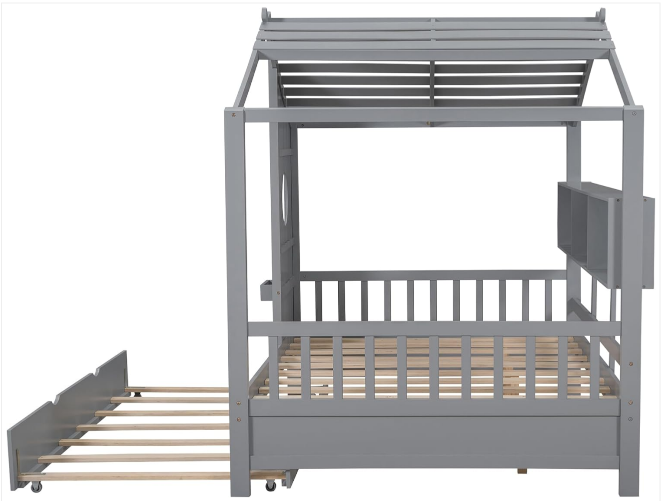
Image 4: Side view of the bed frame, illustrating the connection points for the side rails and the structure of the house-shaped headboard/footboard.
