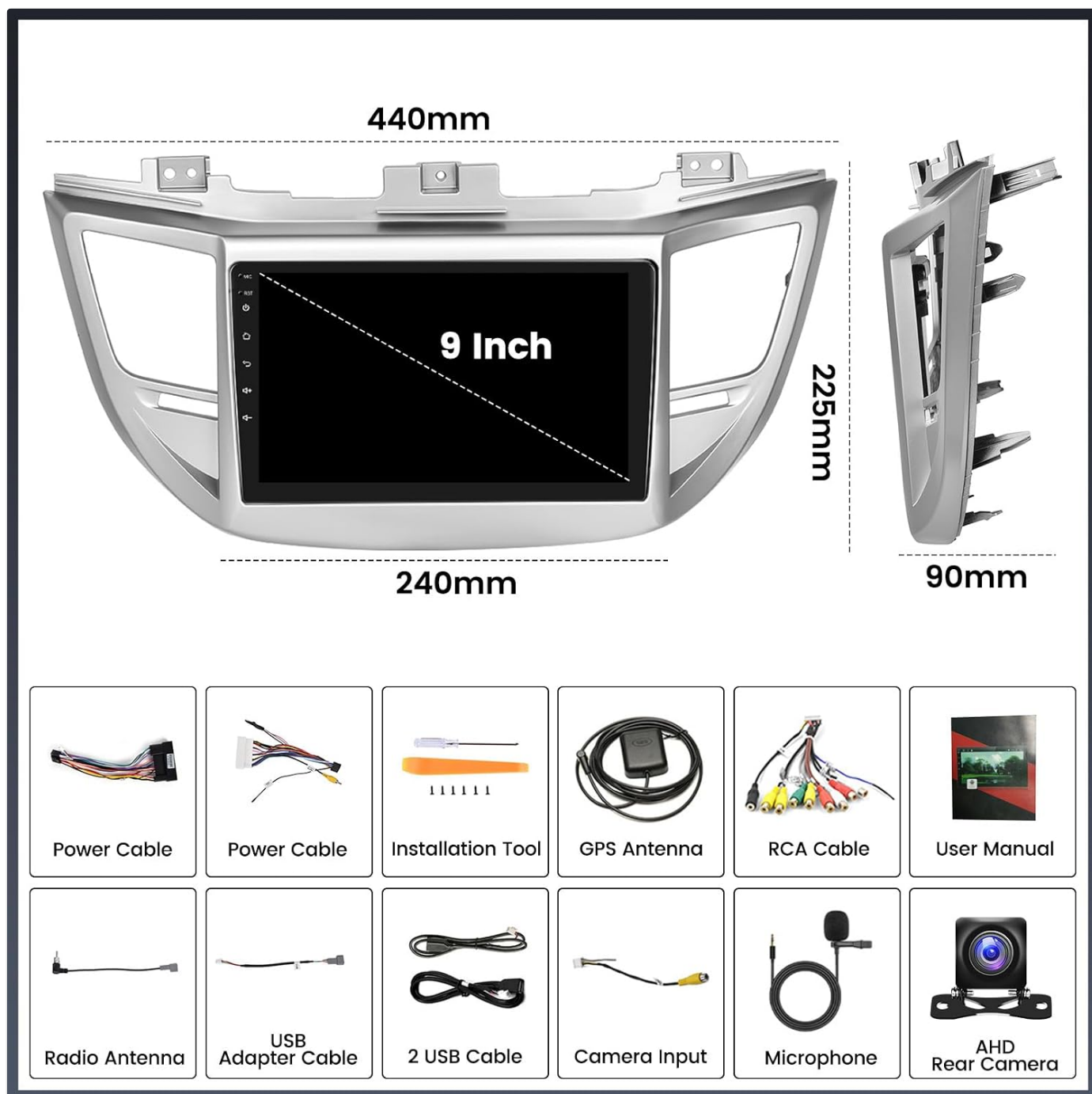
Figure 3.1: Included components and stereo dimensions.
