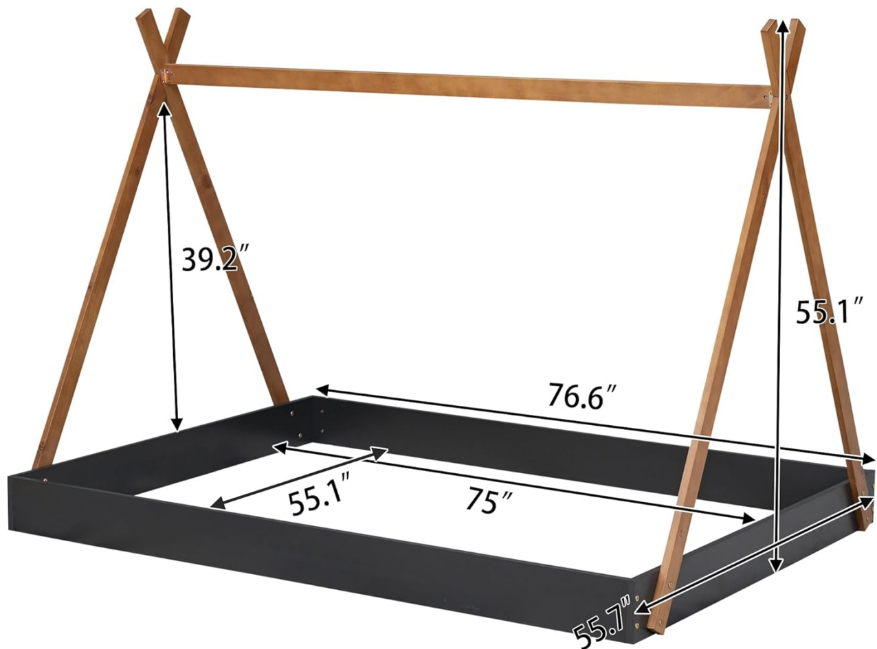
Image: Technical drawing of the Mirightone Full Size Wood Teepee Floor Bed, showing all key dimensions in inches.
