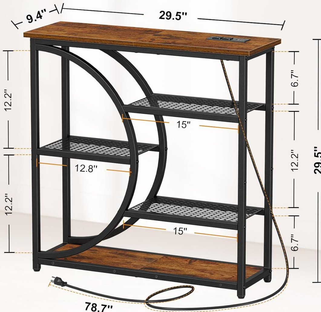
Image: Diagram illustrating the key dimensions of the Snughome Entryway Console Table, including height, width, and depth.
