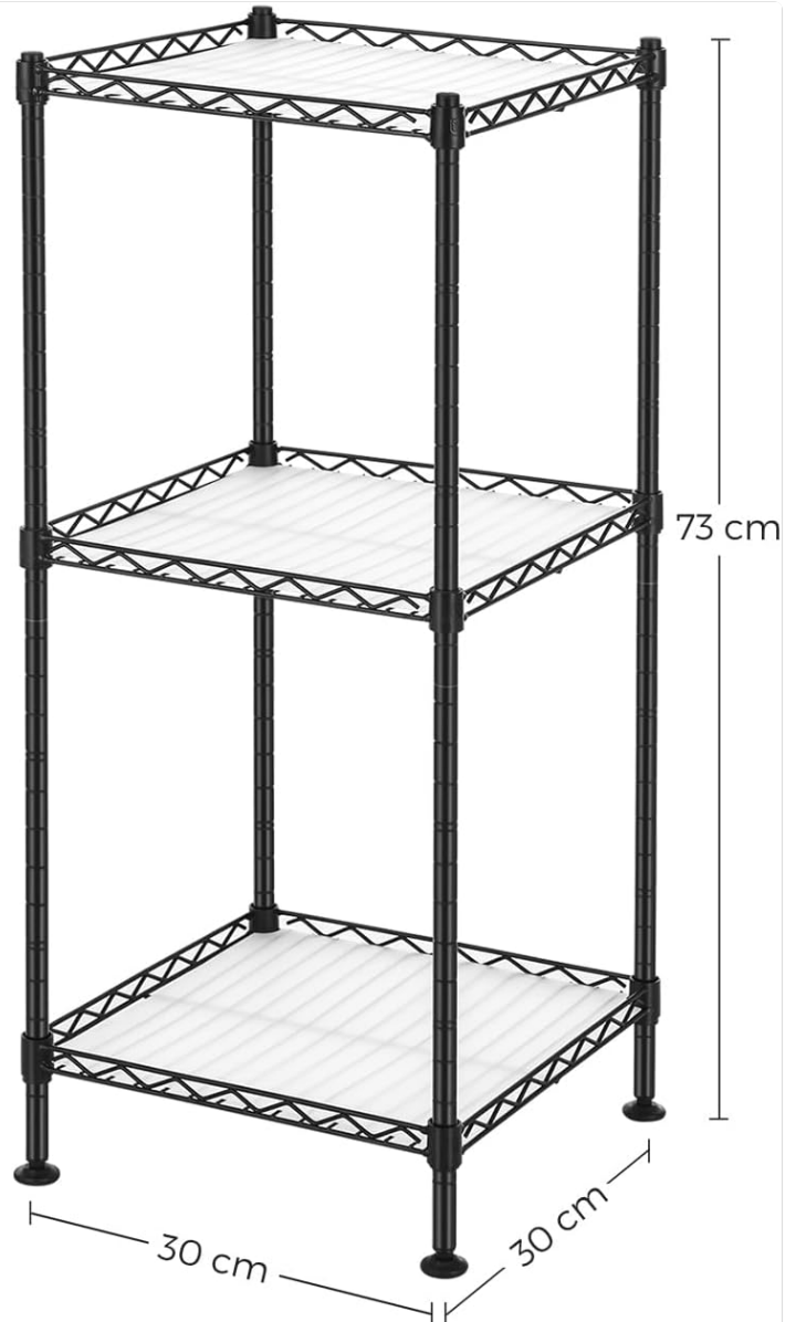
Figure 2: Load capacities and dimensions of the 3-tier rack. Each shelf supports up to 20kg, with a total rack capacity of 65kg.
