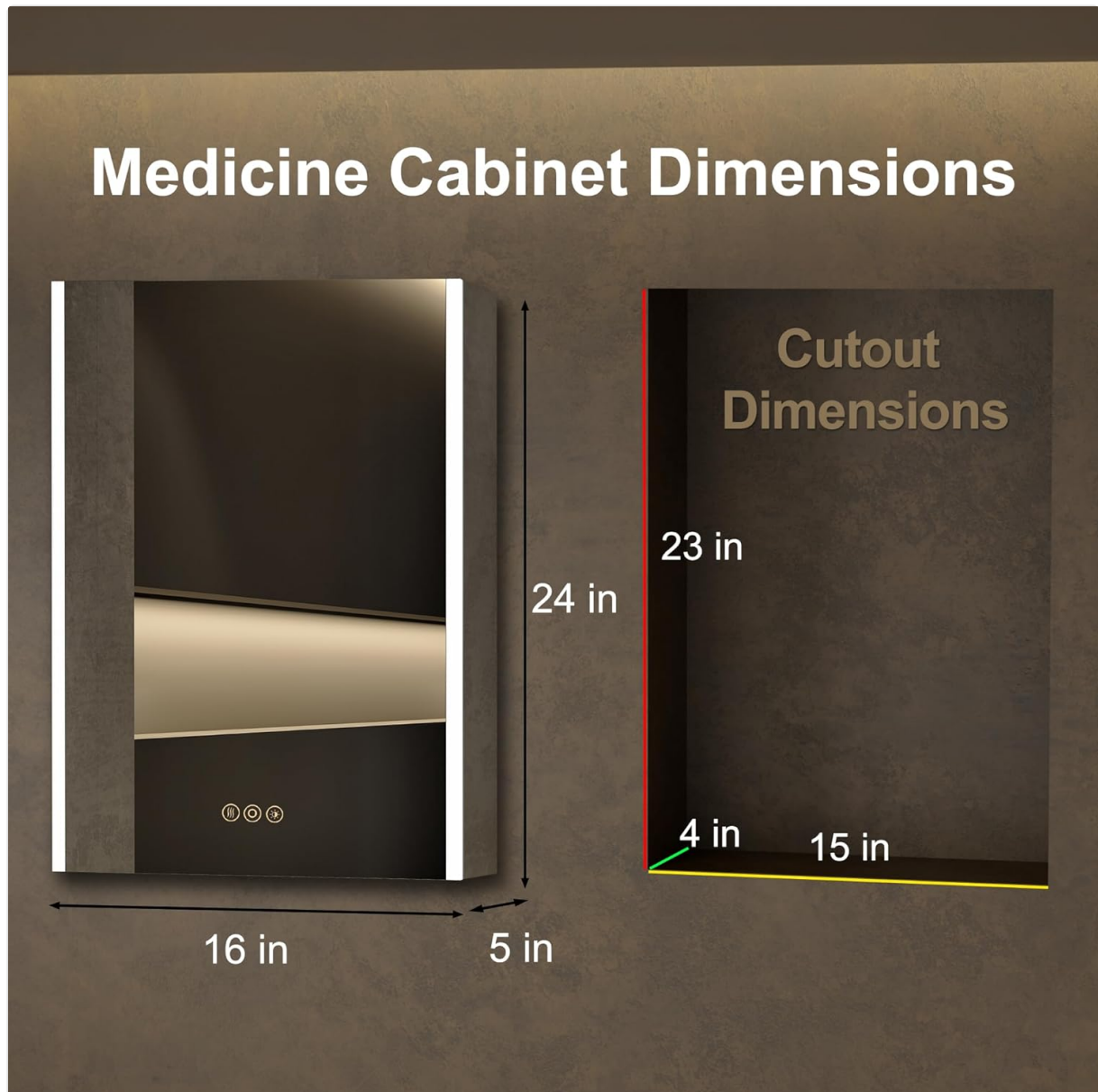
Figure 2: Product dimensions (16 in W x 24 in H x 5 in D) and recommended cutout dimensions for recessed mounting (15 in W x 23 in H x 4 in D).
