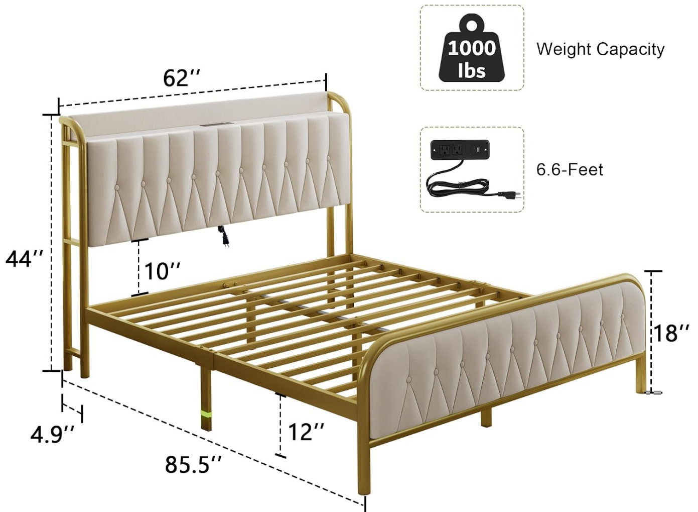
Figure 2.2: Detailed dimensions of the Queen bed frame, including a 1000 lbs weight capacity.
