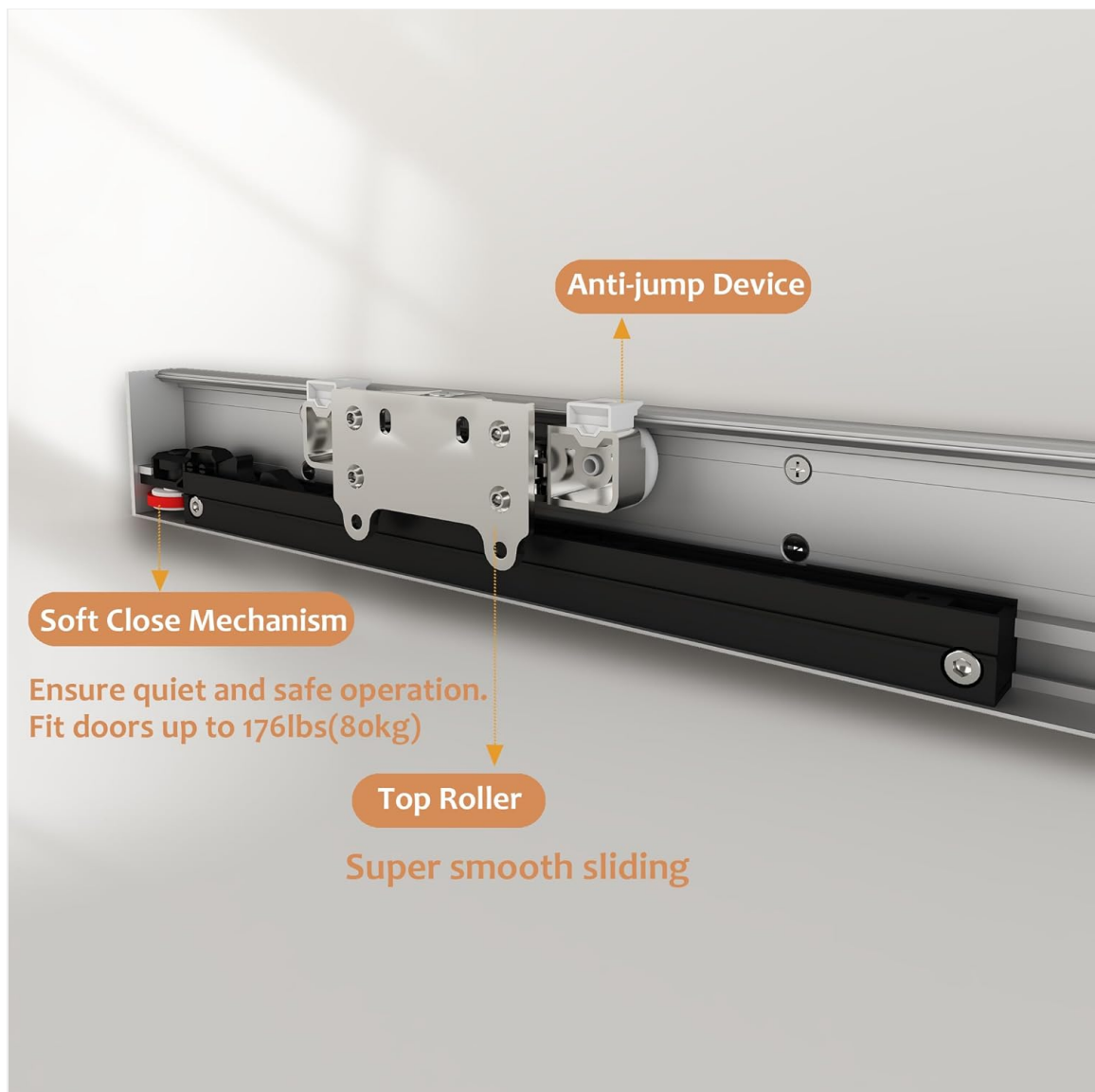
Figure 4: Top track components including soft close mechanism, anti-jump device, and top roller.
