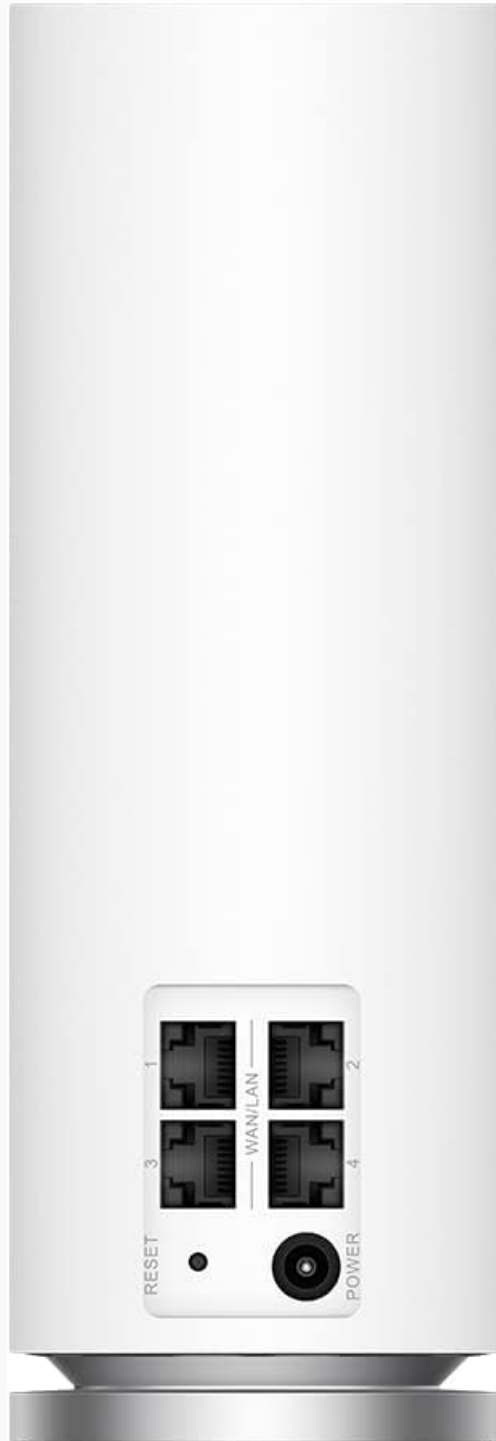
Image: Rear view of the HUAWEI Mesh 7 Router, showing the four Ethernet ports, power input, and reset button.
