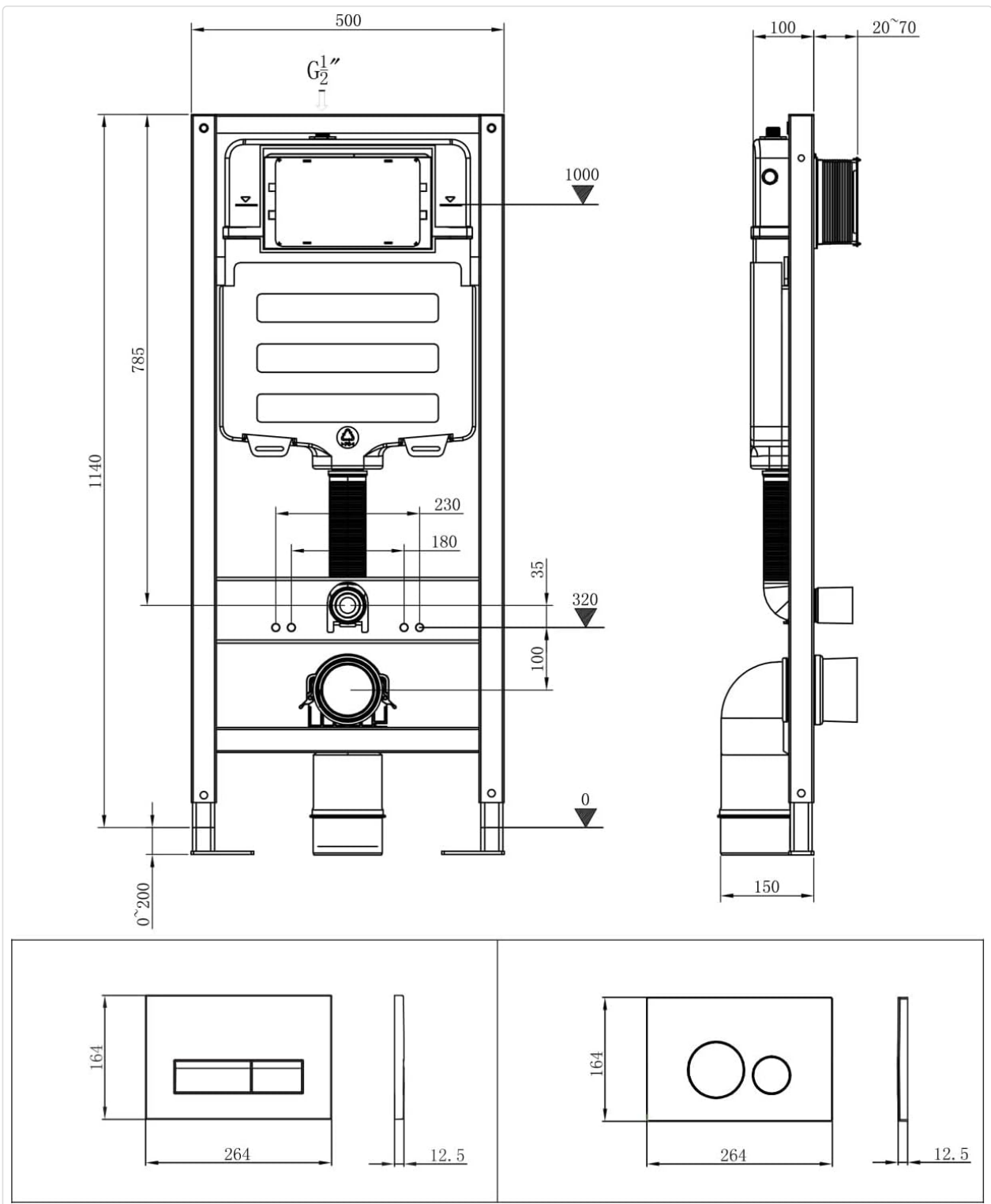
Image: Detailed technical drawing showing the dimensions and internal structure of the concealed toilet tank carrier system.
