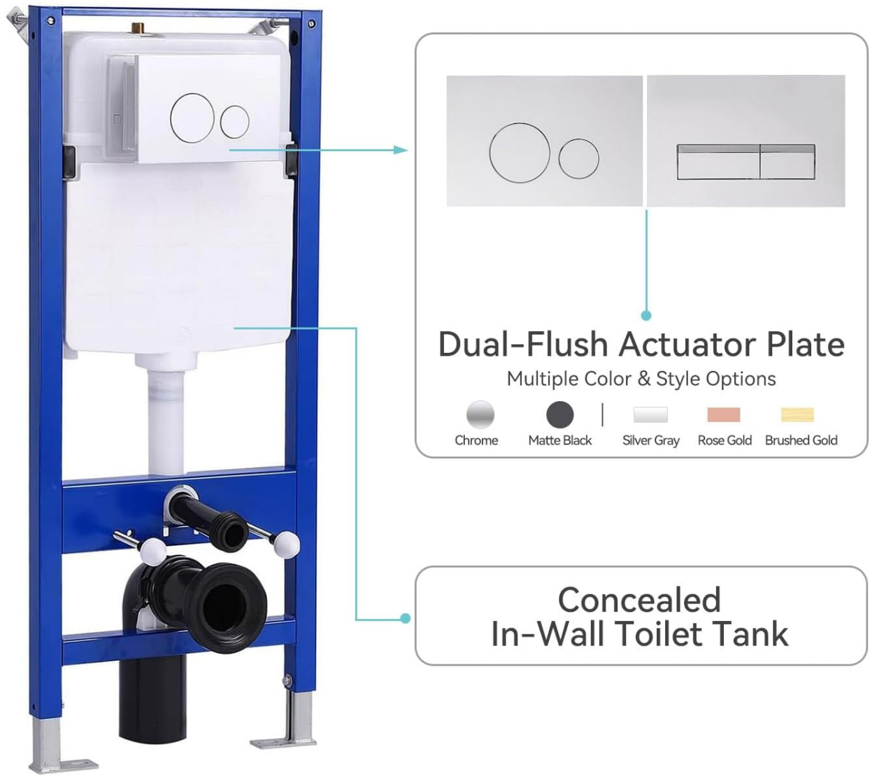
Image: Various styles and colors of the dual-flush actuator plate, showing the two distinct buttons for partial and full flush.
