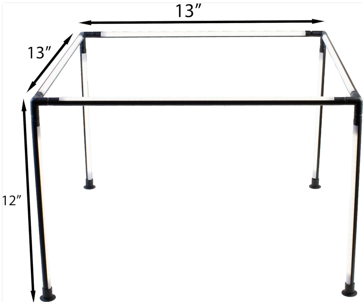
Image: Diagram showing the 13-inch width, 13-inch depth, and 12-inch height dimensions of the LED light frame.
