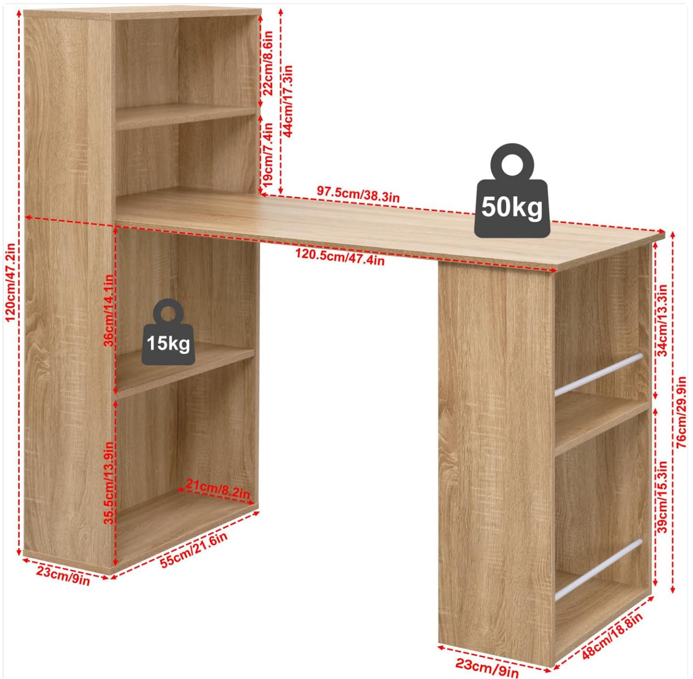
Figure 2: Desk dimensions and weight capacity. The main desktop supports up to 50kg, and the lower shelves support up to 15kg each.
