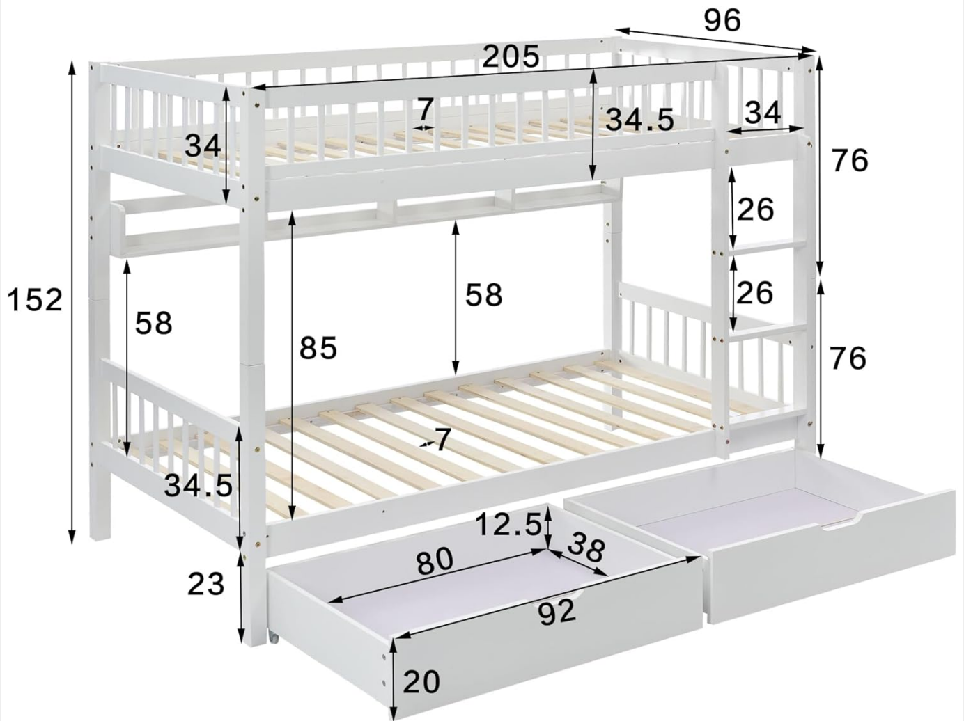
Figure 6: A detailed diagram illustrating the dimensions of the Moimhear Bunk Bed in centimeters, including overall length, width, height, and specific measurements for the ladder, bed separation, and storage drawers.
