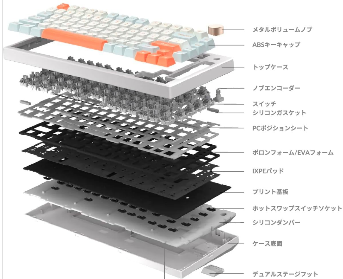
Figure 3.3: An exploded diagram illustrating the multiple buffer layers and components within the VGN N75 keyboard, contributing to its smooth and quiet operation.
