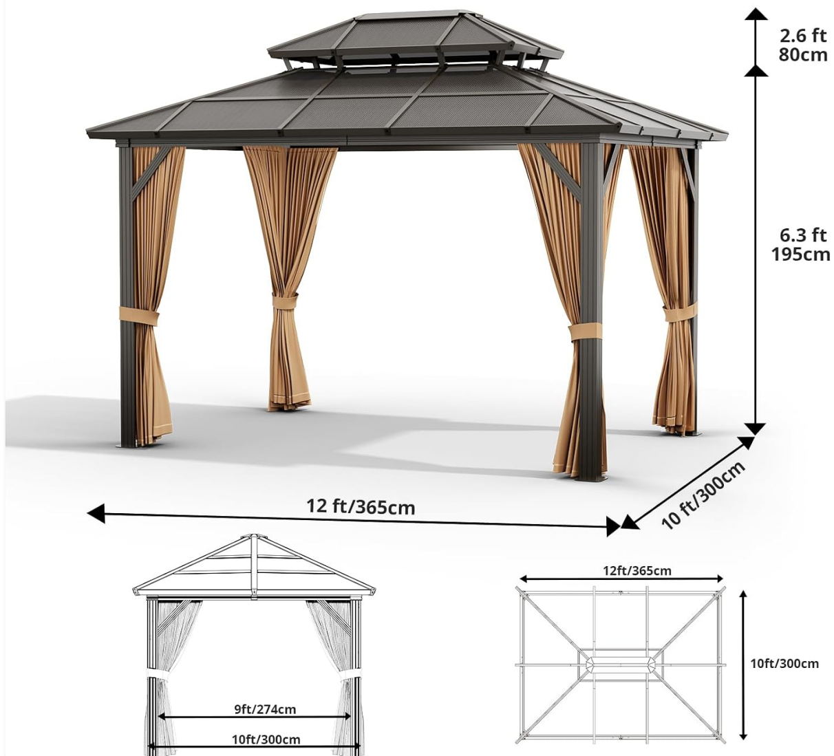
Image: Key dimensions of the GAOMON Hardtop Gazebo.
