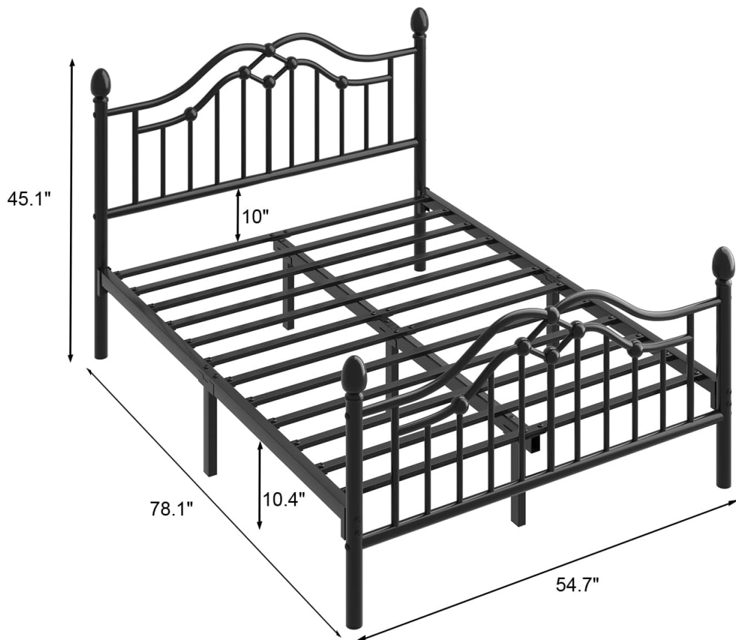
Image: Diagram showing the dimensions of the Full size LOEWAY Metal Bed Frame.
