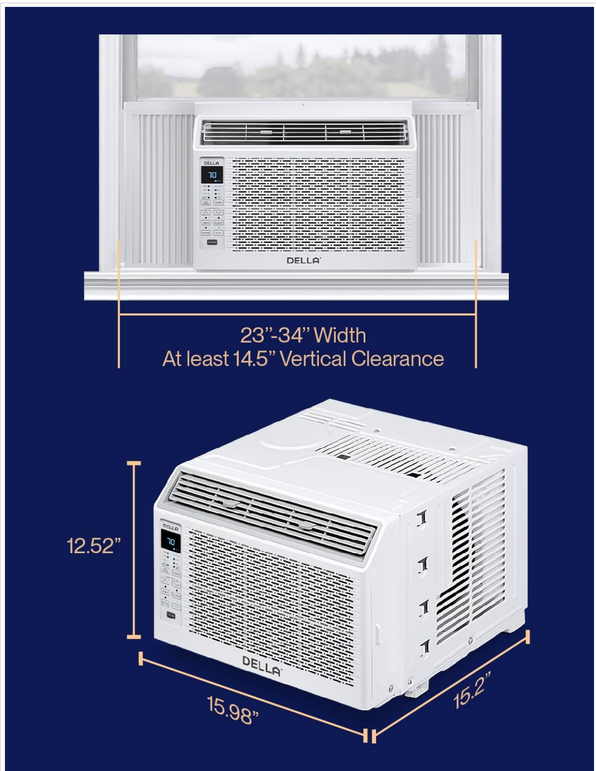
Figure 6: Unit dimensions and recommended window opening.
