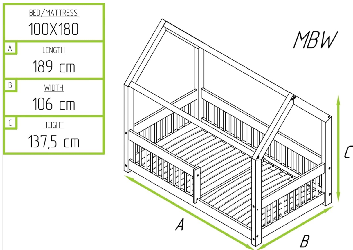
Image 8.1: Dimensional diagram of the ADEKO MBW bed, indicating length (A: 189 cm), width (B: 106 cm), and height (C: 137.5 cm) for a 100x180 cm mattress.
