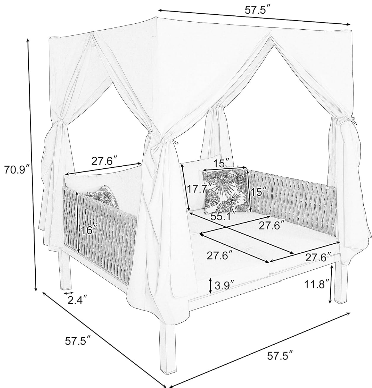
Image: Detailed dimensions of the LUMISOL Outdoor Patio Sunbed.
