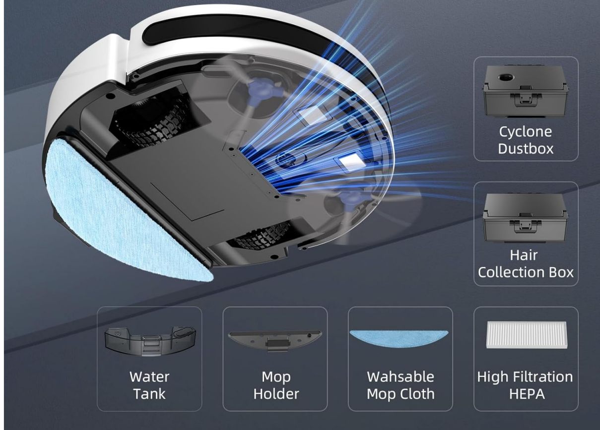
Figure 7: Key components of the Pureatic V3, including the water tank, mop holder, washable mop cloth, and high filtration HEPA filter.
