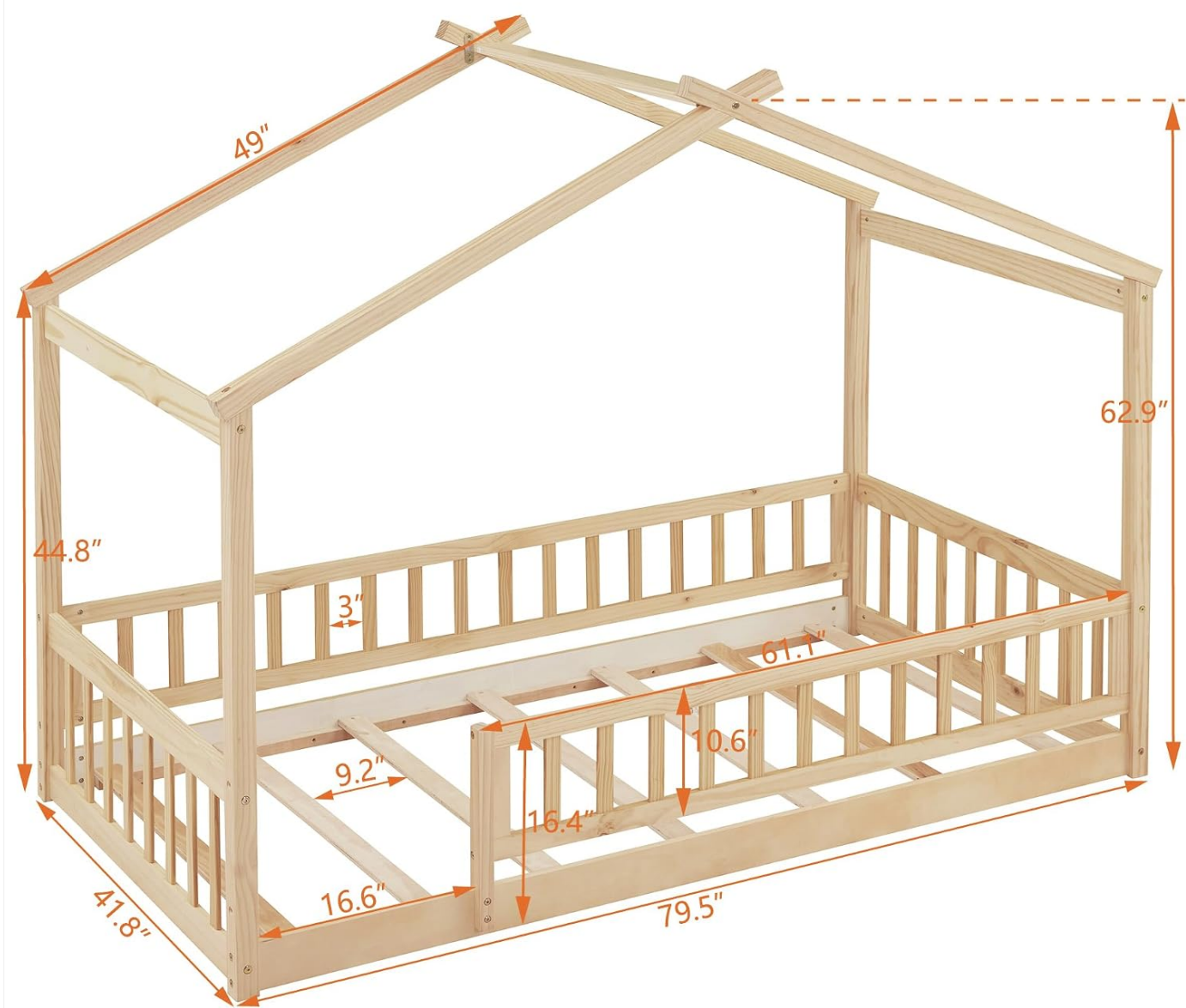
Image: Detailed dimensions of the bed frame.
