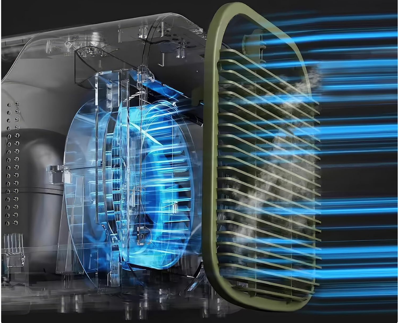
Figure 1.2: High cooling efficiency with upgraded air duct system and piston compressor.
