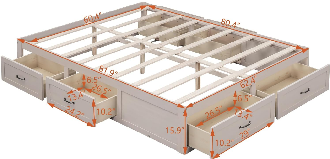
Image 8.1: A technical diagram illustrating the precise dimensions of the Mirightone Queen Storage Platform Bed, including overall length, width, height, and internal drawer measurements.
