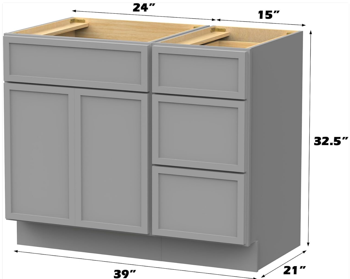
Figure 3.1: Product dimensions for planning installation.
