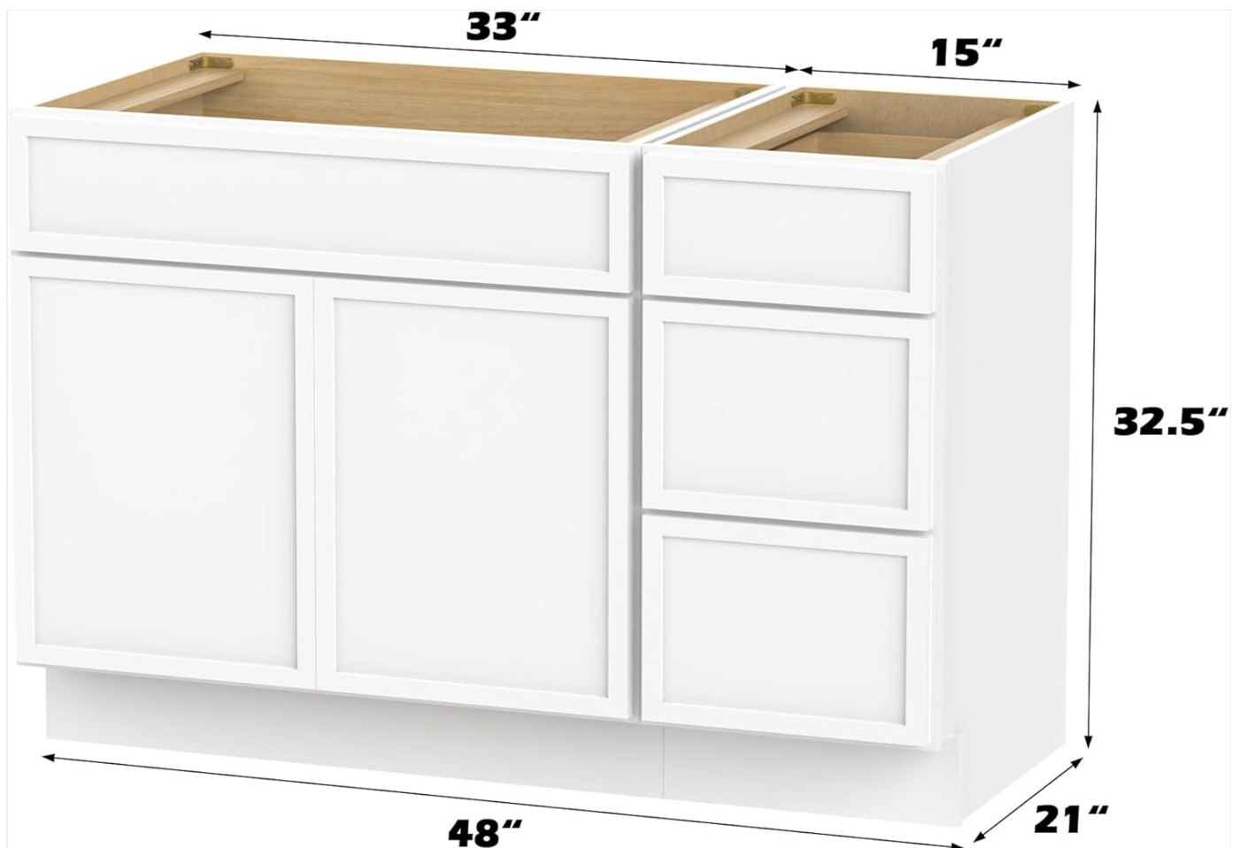
Image 4.1: Dimensions of the unassembled vanity for planning purposes.
