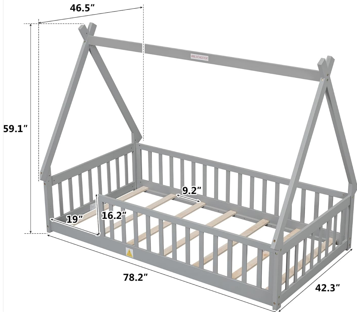
Figure 4.1: Product Dimensions. This diagram provides key measurements (78.2"L x 46.5"W x 59.1"H) and internal dimensions, crucial for understanding the bed's structure during assembly.
